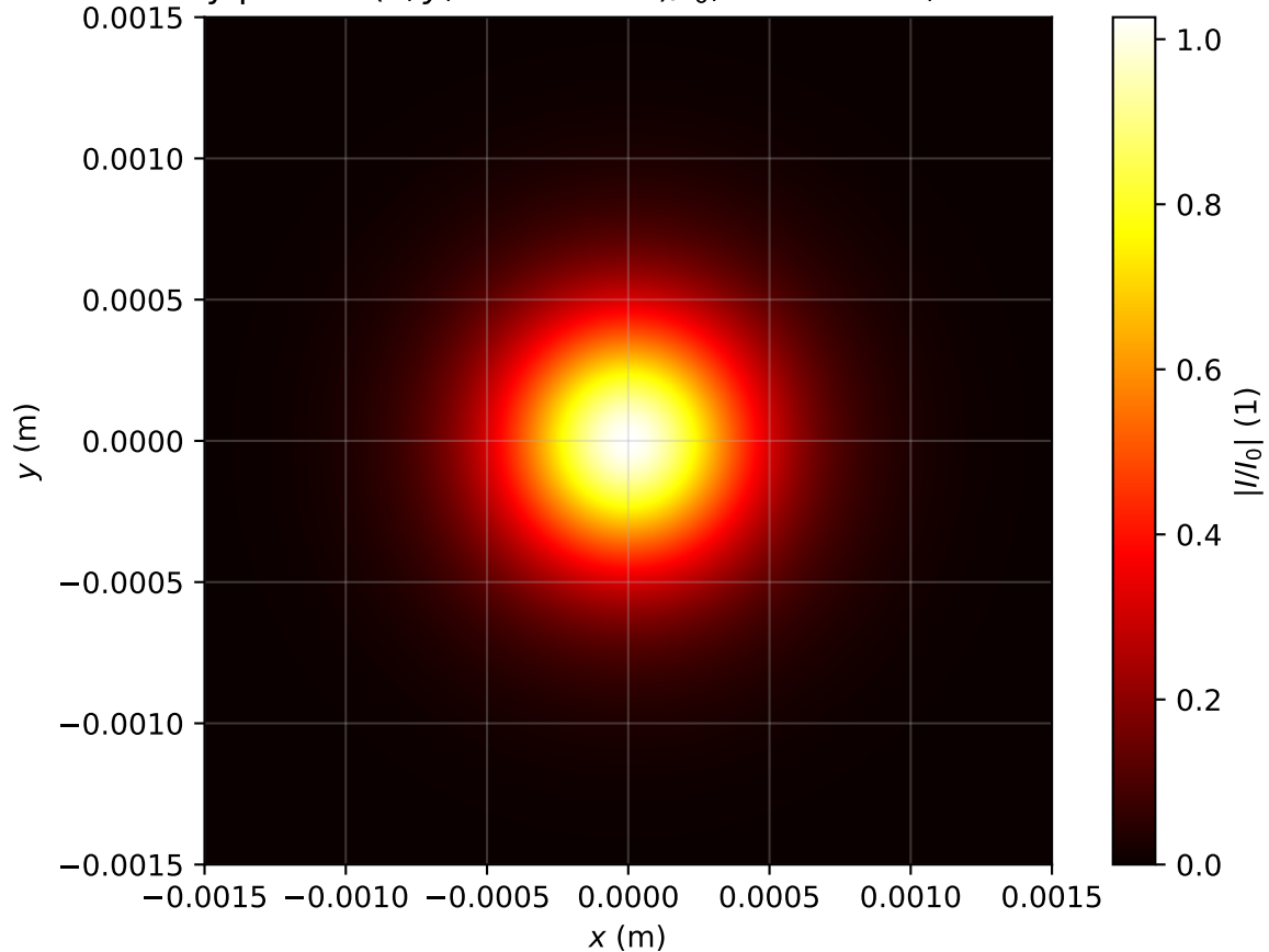
Intensity profile I(x, y, z = 1.672m)/I_0 , Pin=0.6Pcr, artificial time
